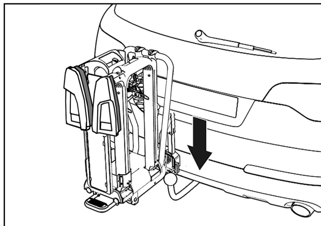
Fig. 9: Attaching the carrier to the trailer couplin
