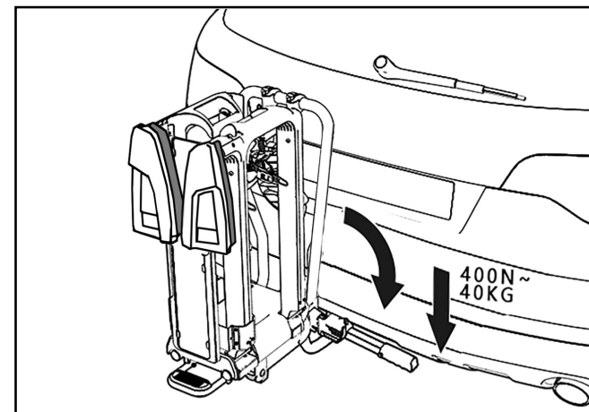
Figure 10: Closing the quick-release fastener
