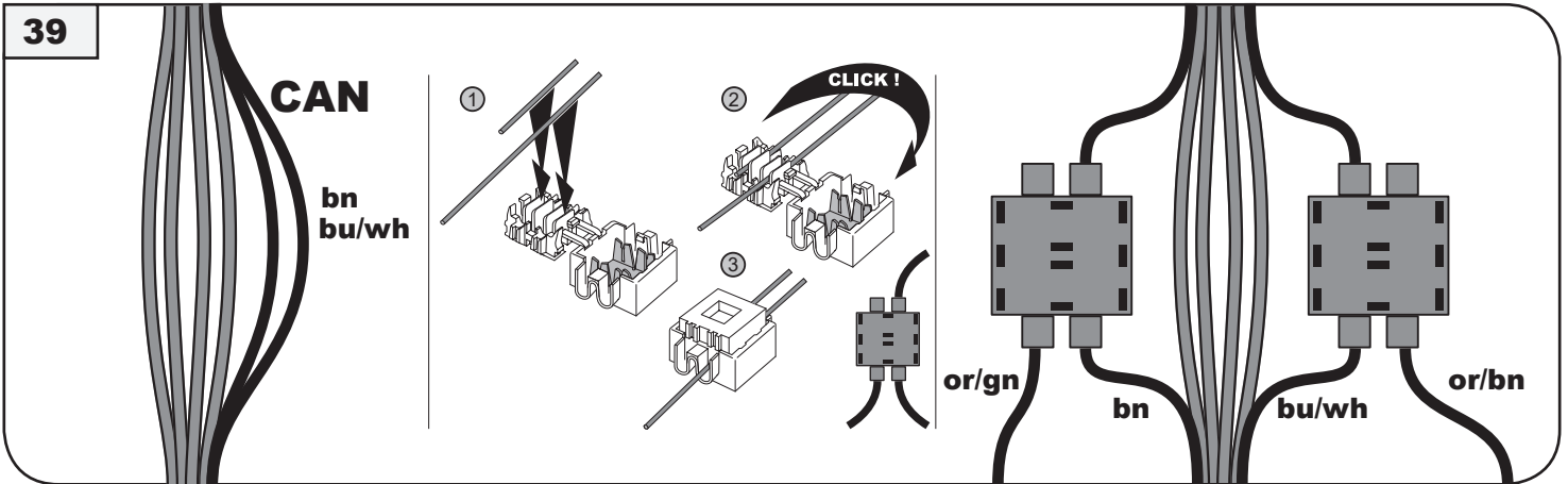
E-Satz or/gn → kabel bn, E-Satz or/bn → kabel bu/wh e-kit or/gn → cabel car bn, e-kit or/bn → cabel car bu/wh
