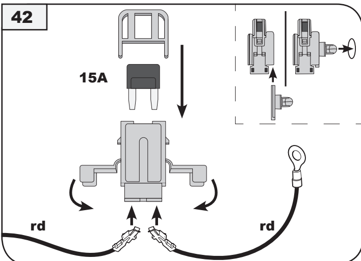
Modul Trail-tec 30-10 LED → Stecker 14 pin E-Satz modul Trail-tec 30-10 LED → socket 14 pin e-kit
