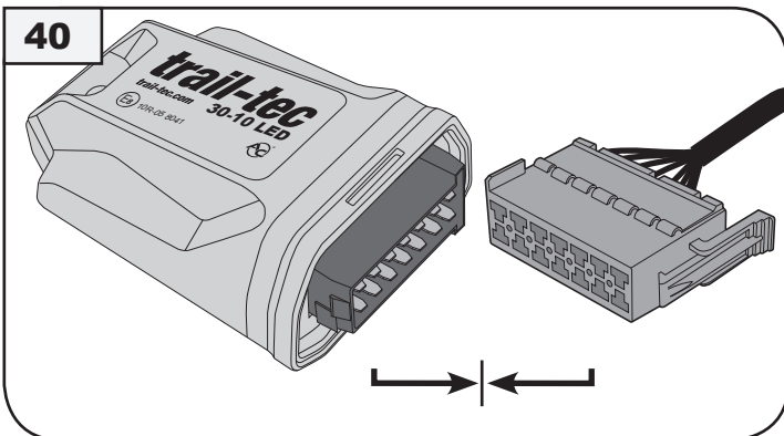
Modul Trail-tec 30-10 LED → Stecker 14 pin E-Satz modul Trail-tec 30-10 LED → socket 14 pin e-kit
