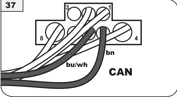
E-Satz Stecker (bn pin 5, bu/wh pin 6) e-kit socket (bn pin 5, bu/wh pin 6)
